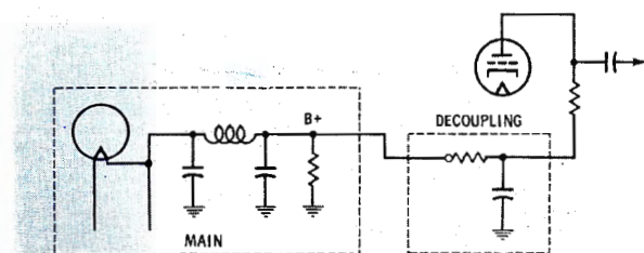
Fig. 1. Power supply—main B+ and decoupling networks.
