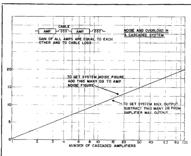
Fig. 3. Relation of number of amplifiers to noise figure.
