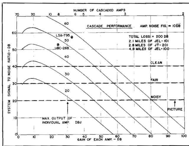
Fig. 5. Curves for 10 db noise figure and 200 db loss.
