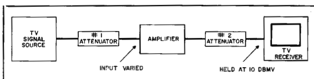
Fig. 1. Basic wide-band television distribution system.
